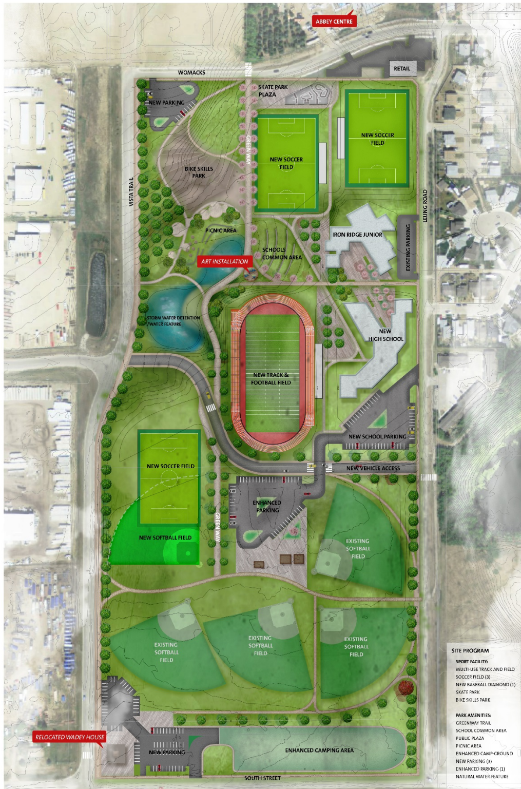
Figure 4-1: Concept Plan
